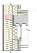
2. INTERMEDIATE FLOOR
