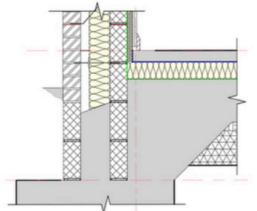
4. MASONRY FOUNDATION
